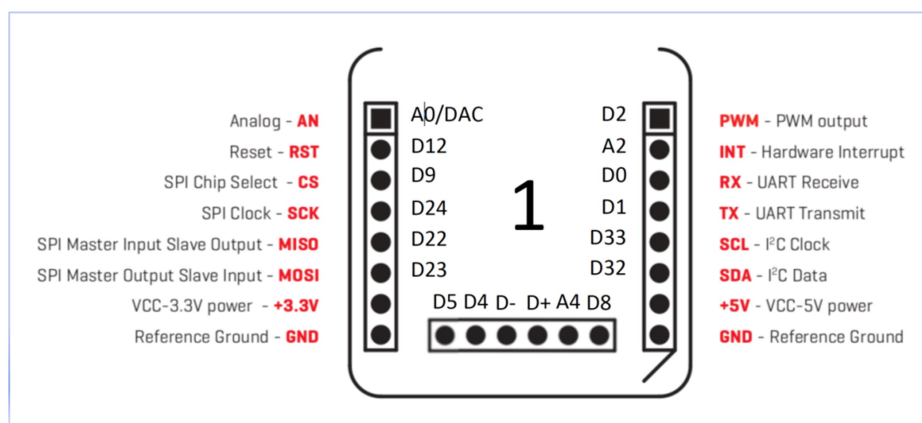
pin out connector 1 Arancino
