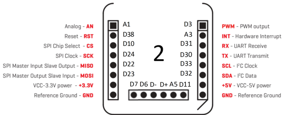
fig 5 arancino connector 2
