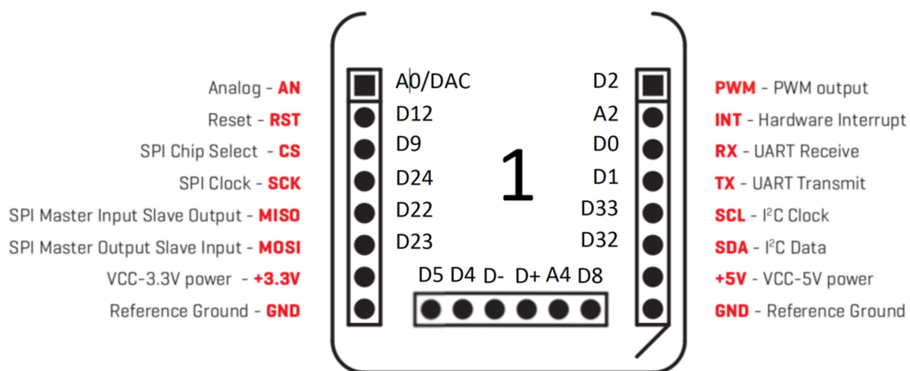
fig. 4: arancino connector 1
